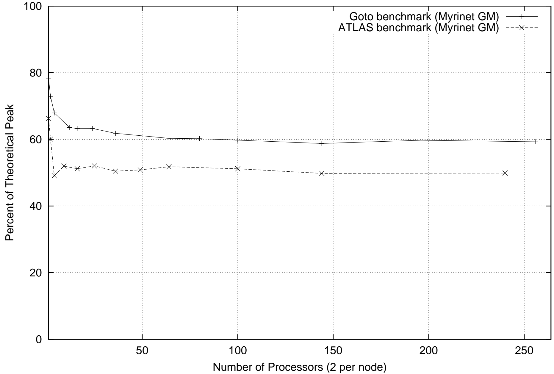
Aspen Systems Linux Cluster Pentium4 XeonDP 2 GHz HPL Performance (gcc -O3)
