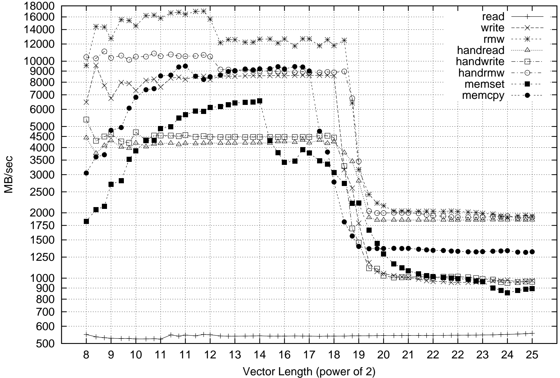
Aspen Systems Linux Pentium4XeonDP 2 GHz Memory Hierarchy Performance (icc -O2)
