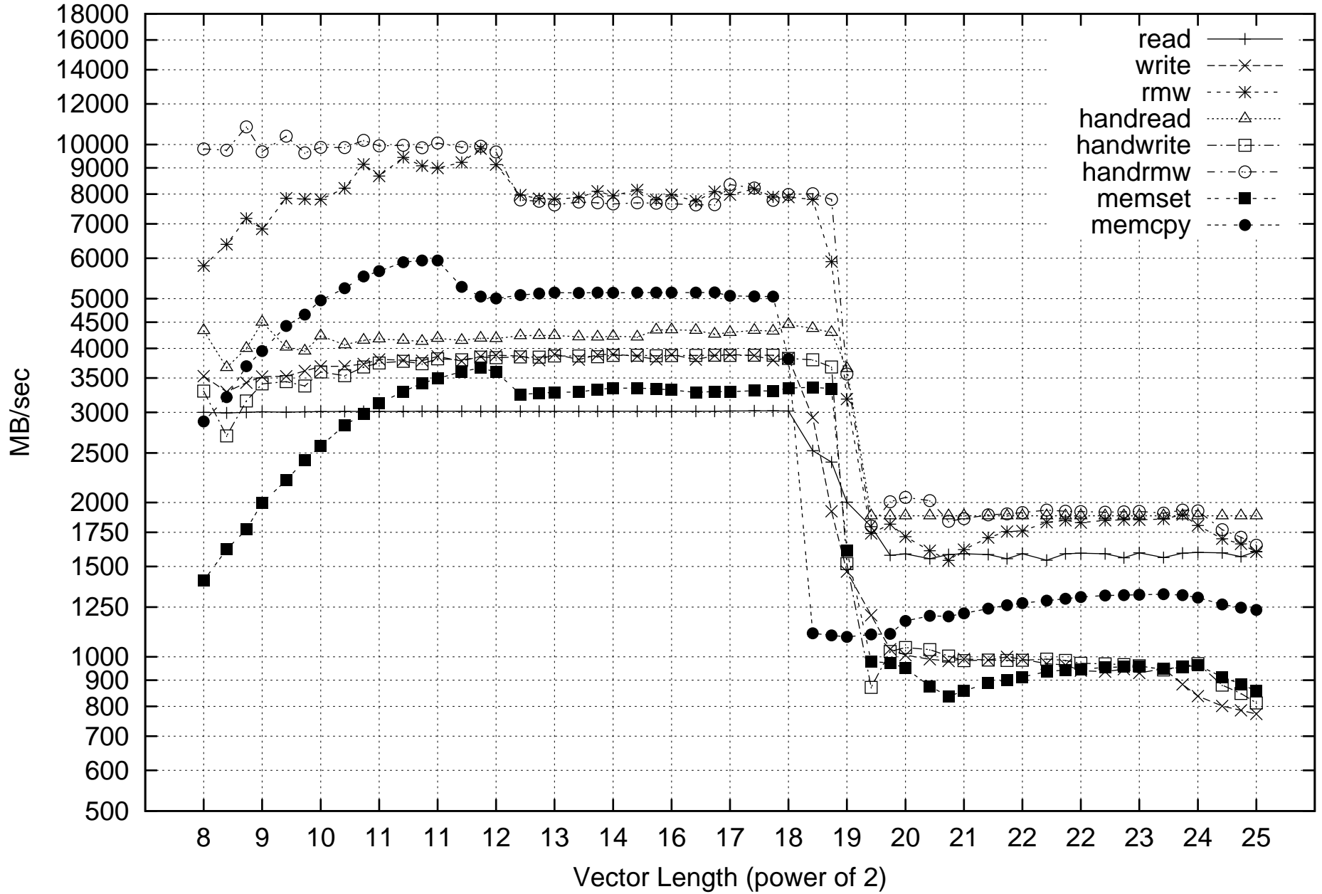
Aspen Systems Linux Pentium4XeonDP 2 GHz Memory Hierarchy Performance (gcc -O3)
