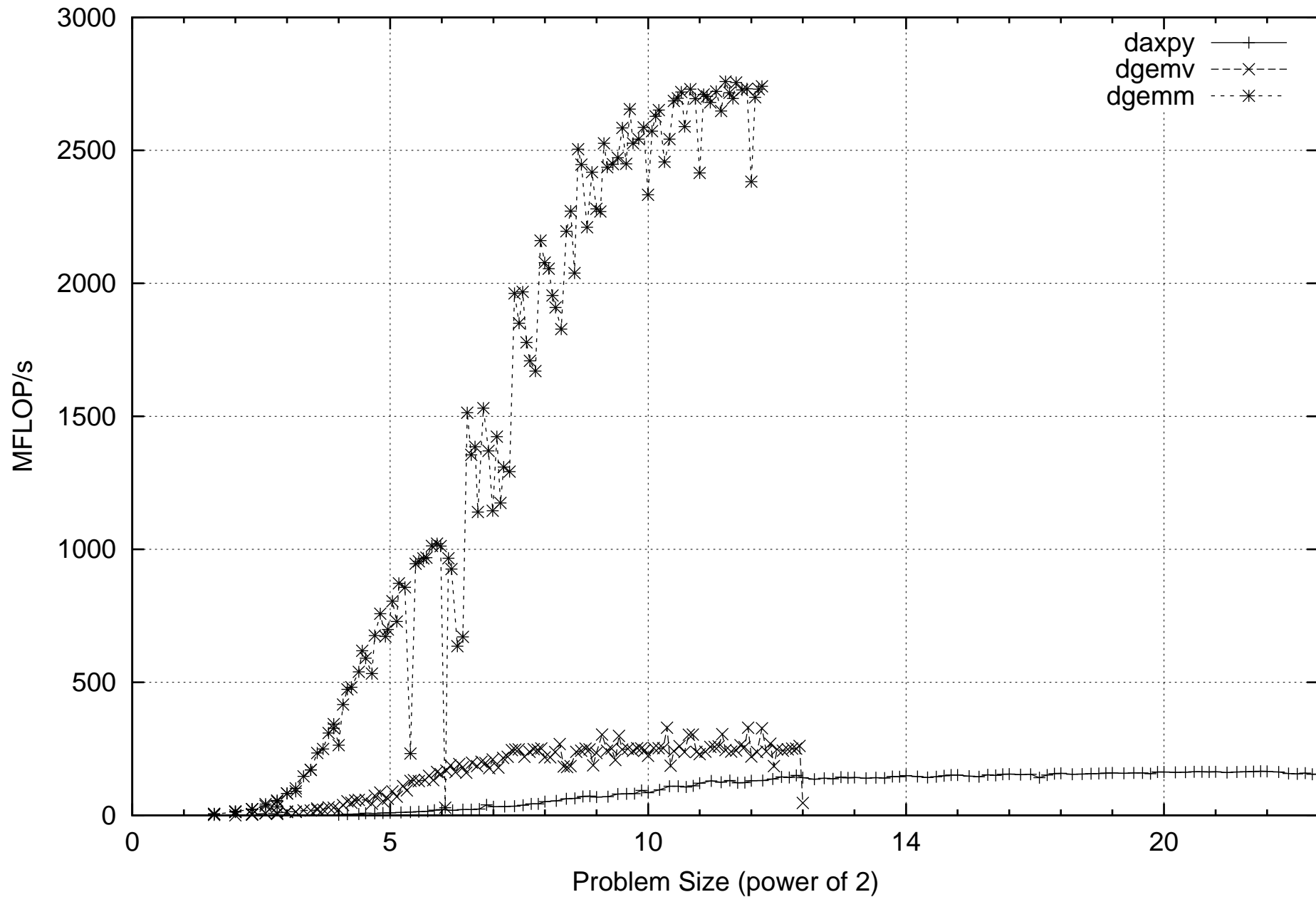
Aspen Systems Linux Pentium4 Xeon 2 GHz ATLAS BLAS Performance (gcc -O3)
