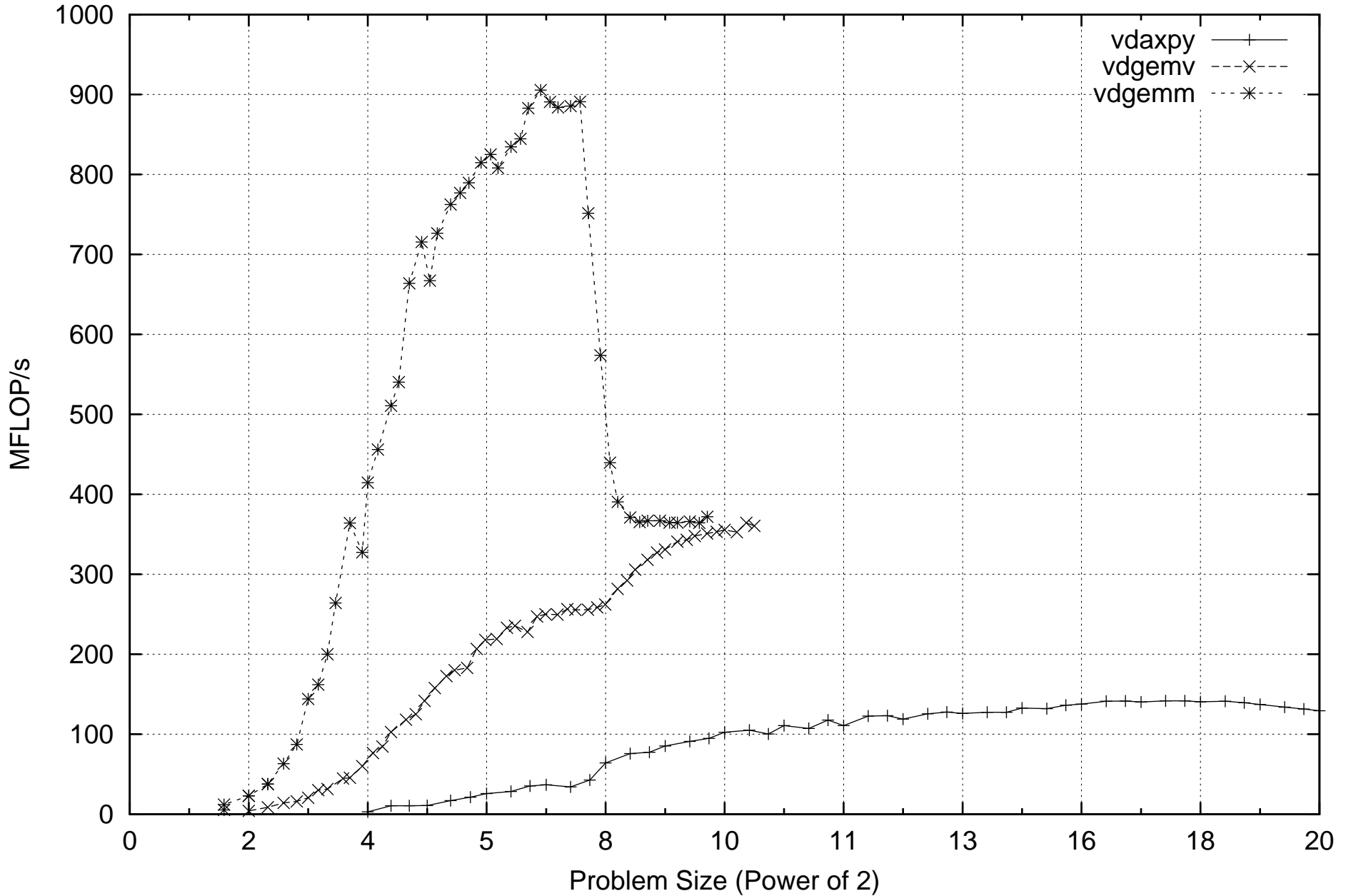
Aspen Systems Linux Pentium4Xeon Cluster Netlib BLAS Performance (gcc -O3)
