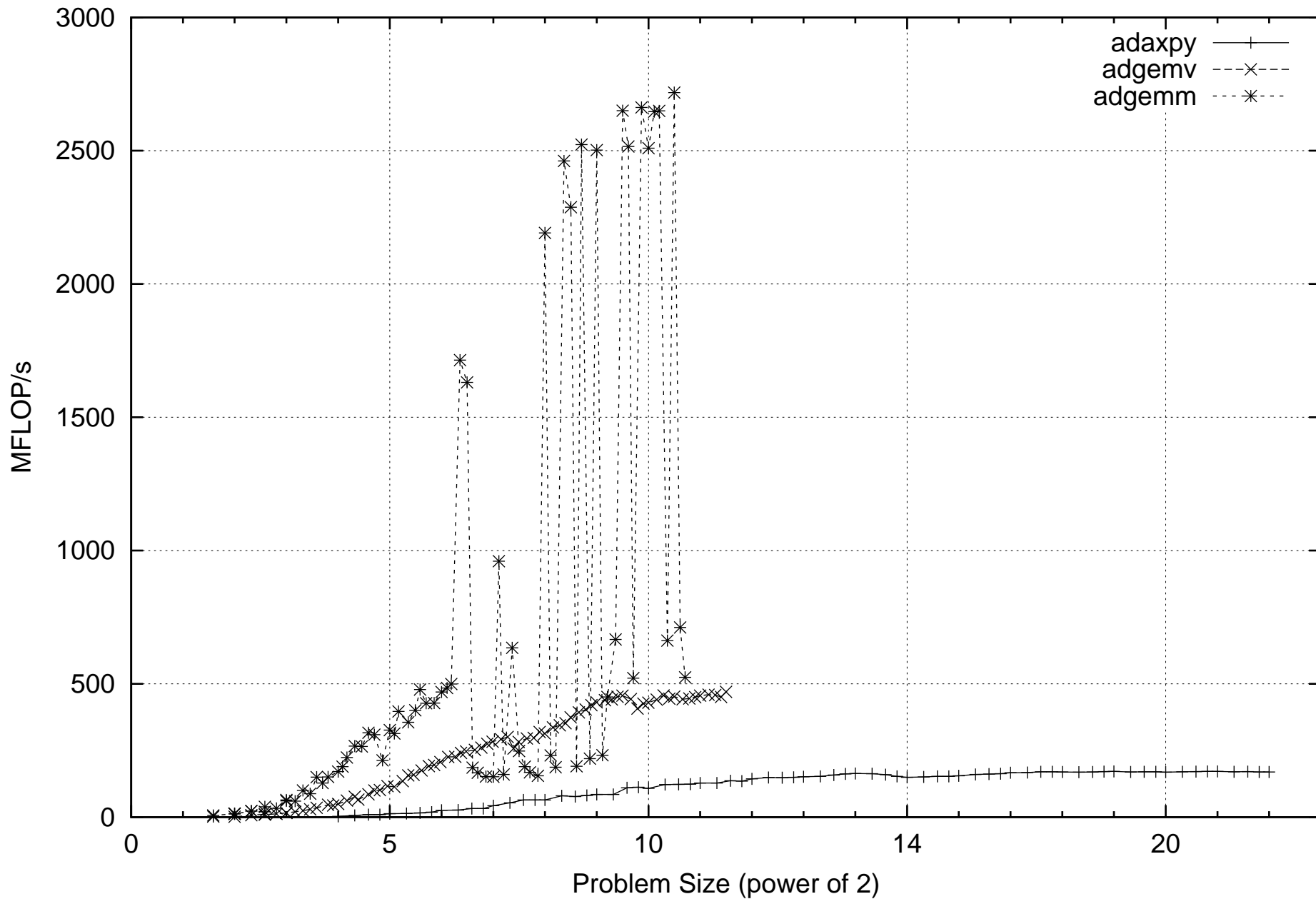
Aspen Systems Linux Pentium4 Xeon 2 GHz ATLAS BLAS Performance (icc -O2)
